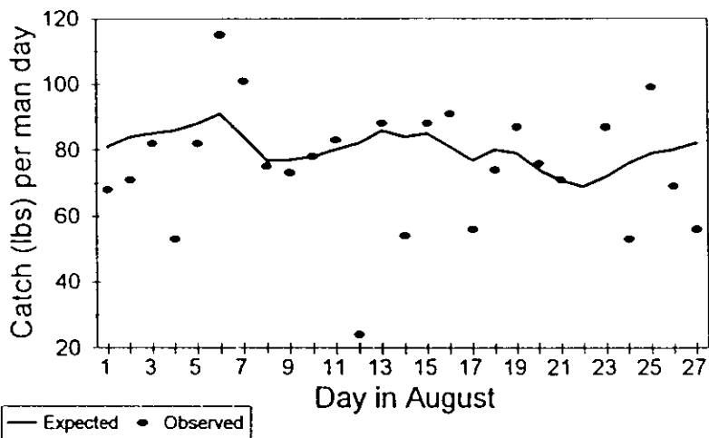
Figure 5. Observed and expected CPUE for August 1979 using the CEDA constant recruitment model ( M = 0.05 ; Initial Proportion = 0.5). There was no initial decline in CPUE, explained by fishing before 1st August.
